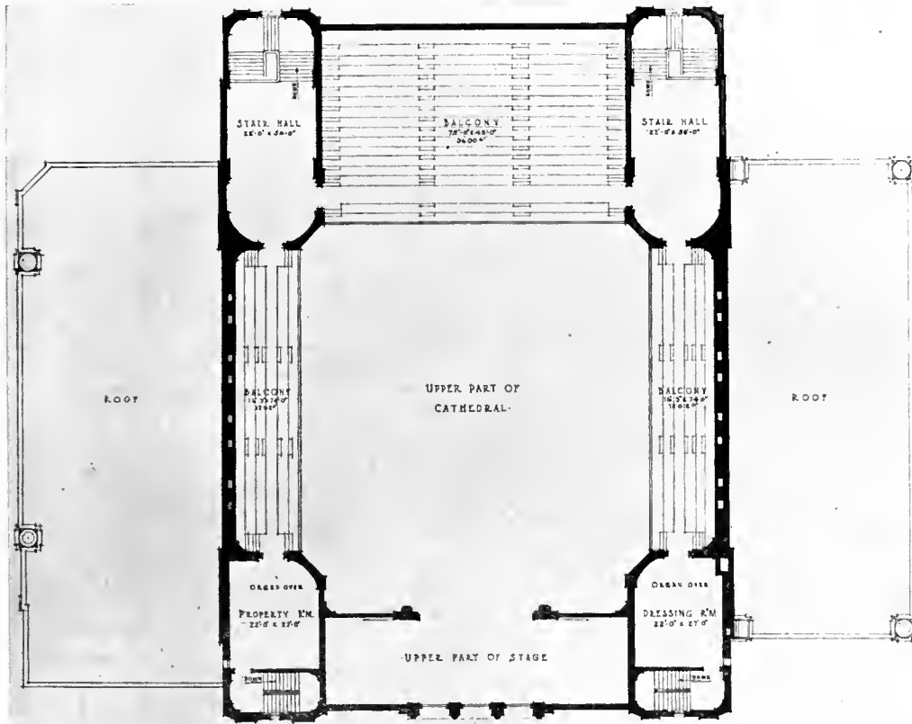
BALCONY FLOOR PLAN
